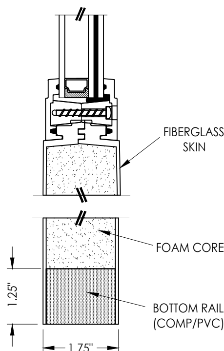
2 VERTICAL CROSS SECTION 3
